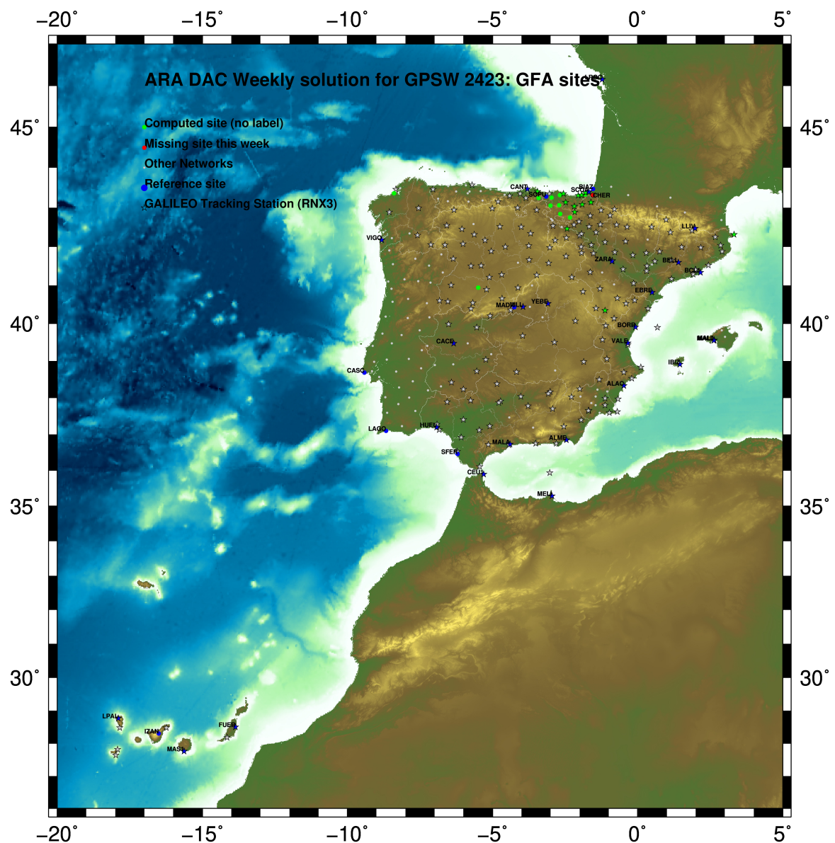
Fig.1: Computed Sites for GPS Week2423 (GFA)
