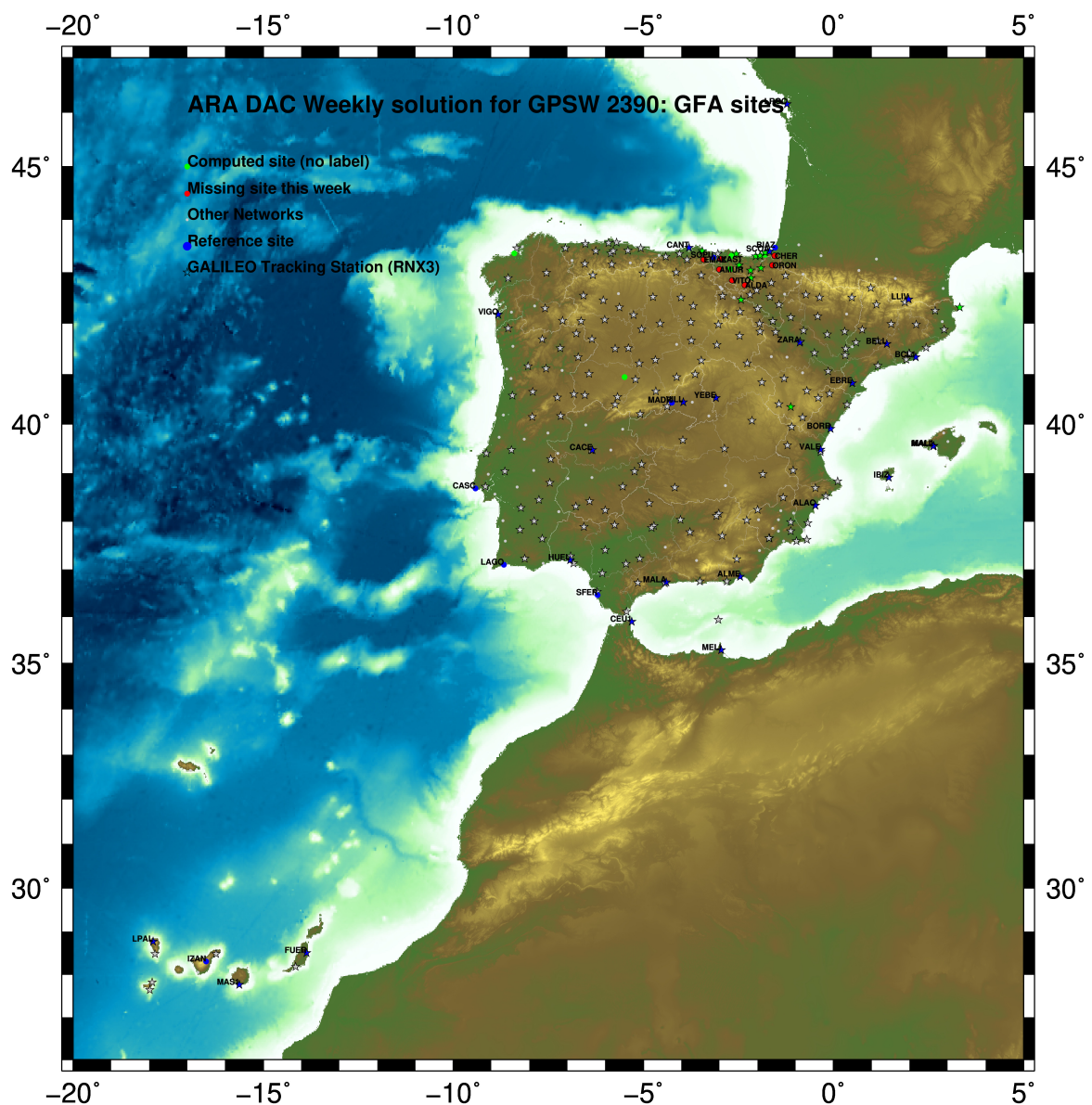
Fig.1: Computed Sites for GPS Week2390 (GFA)
