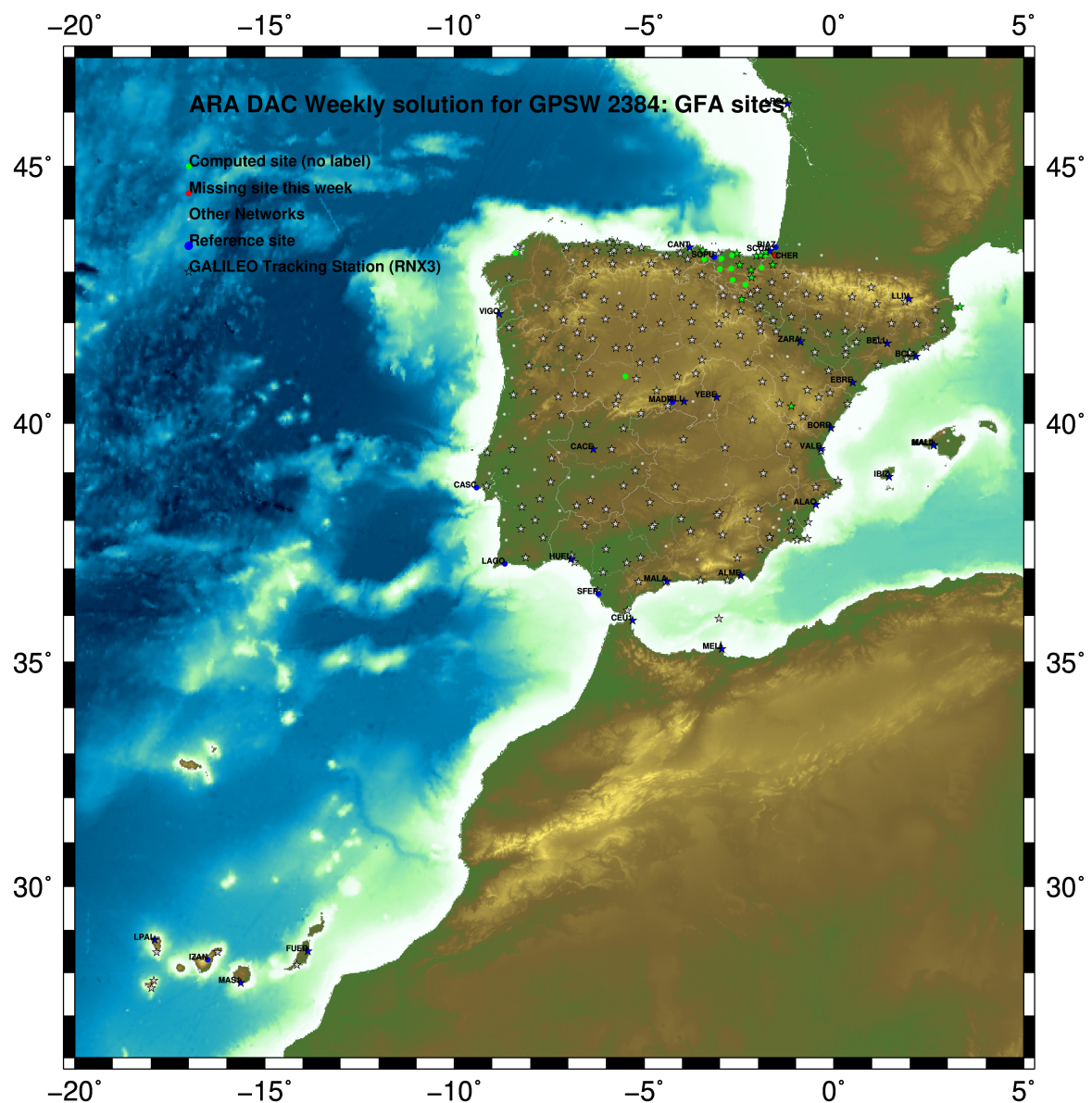
Fig.1: Computed Sites for GPS Week2384 (GFA)
