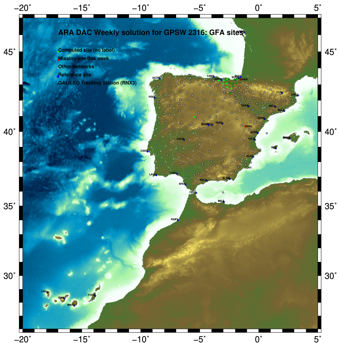
Fig.1: Computed Sites for GPS Week2316 (GFA)
