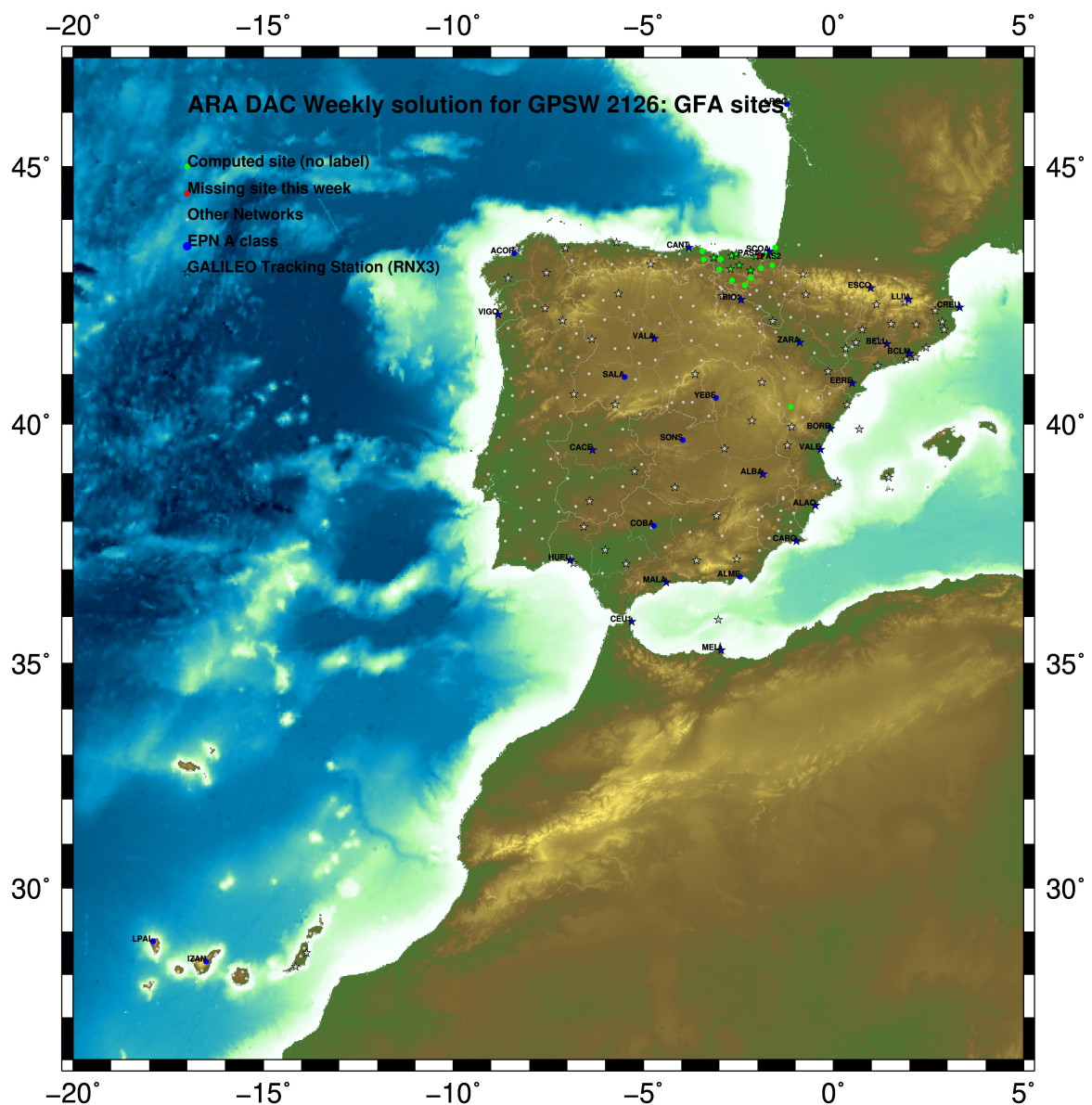
Fig.1: Computed Sites for GPS Week2126 (GFA)
